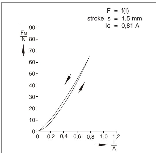
Bild 7: Force/current-characteristic with constant stroke Typ G RF Y 045 F20 B01
