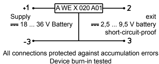
Fig. 4: block diagram A WE X 020 A01
