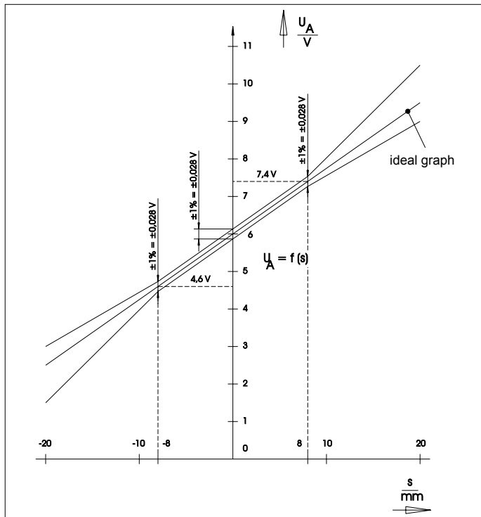
Fig. 2: characteristic A WE X 020 A01
