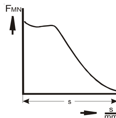
Fig. 2: Magnetic force vs stroke graph
