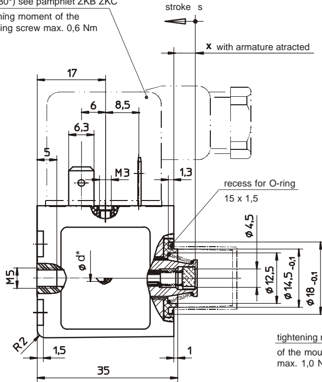
Fig. 5: Type X BK K 032 K54 A01 to A06 * types A03 and A06 without thread M5 and ∅ d (see fig. 10)
