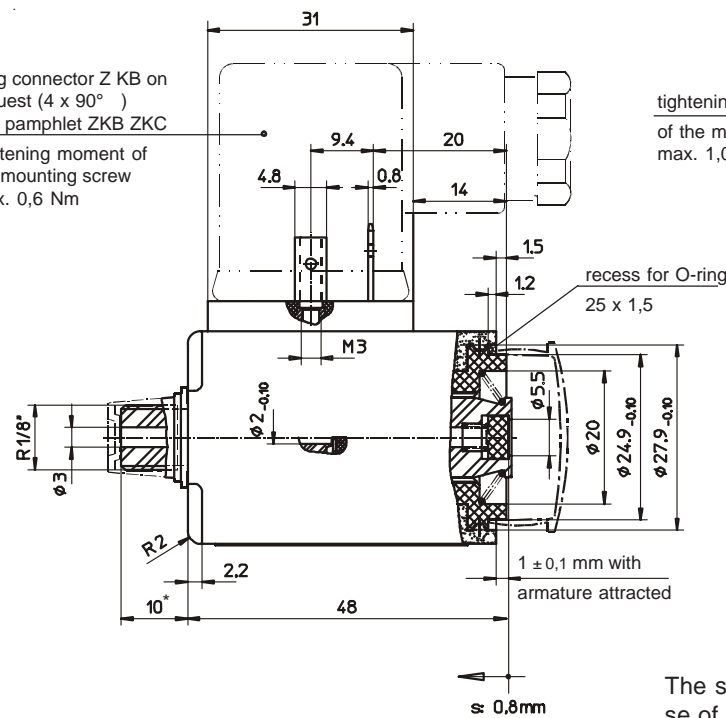
Fig. 6: Type X BK K 032 K54 A01 to A03 * type A03 without thread R 1/8" (see fig. 10)
